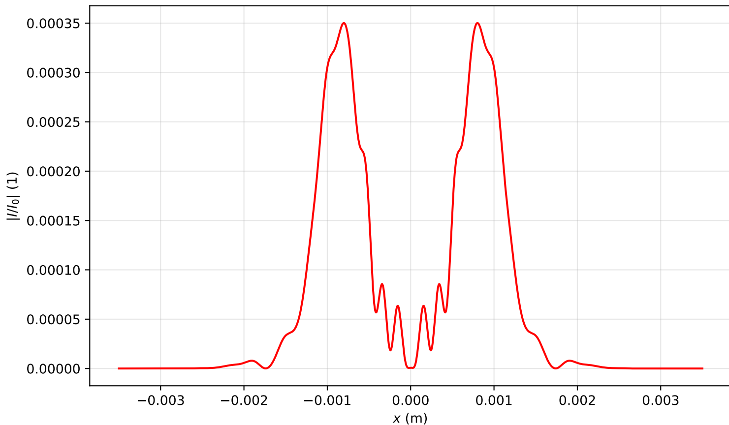
Intensity profile I(x, y = 0, z = 1.035)/I_0 , P_{in}=8.0P_{cr} , artificial time
